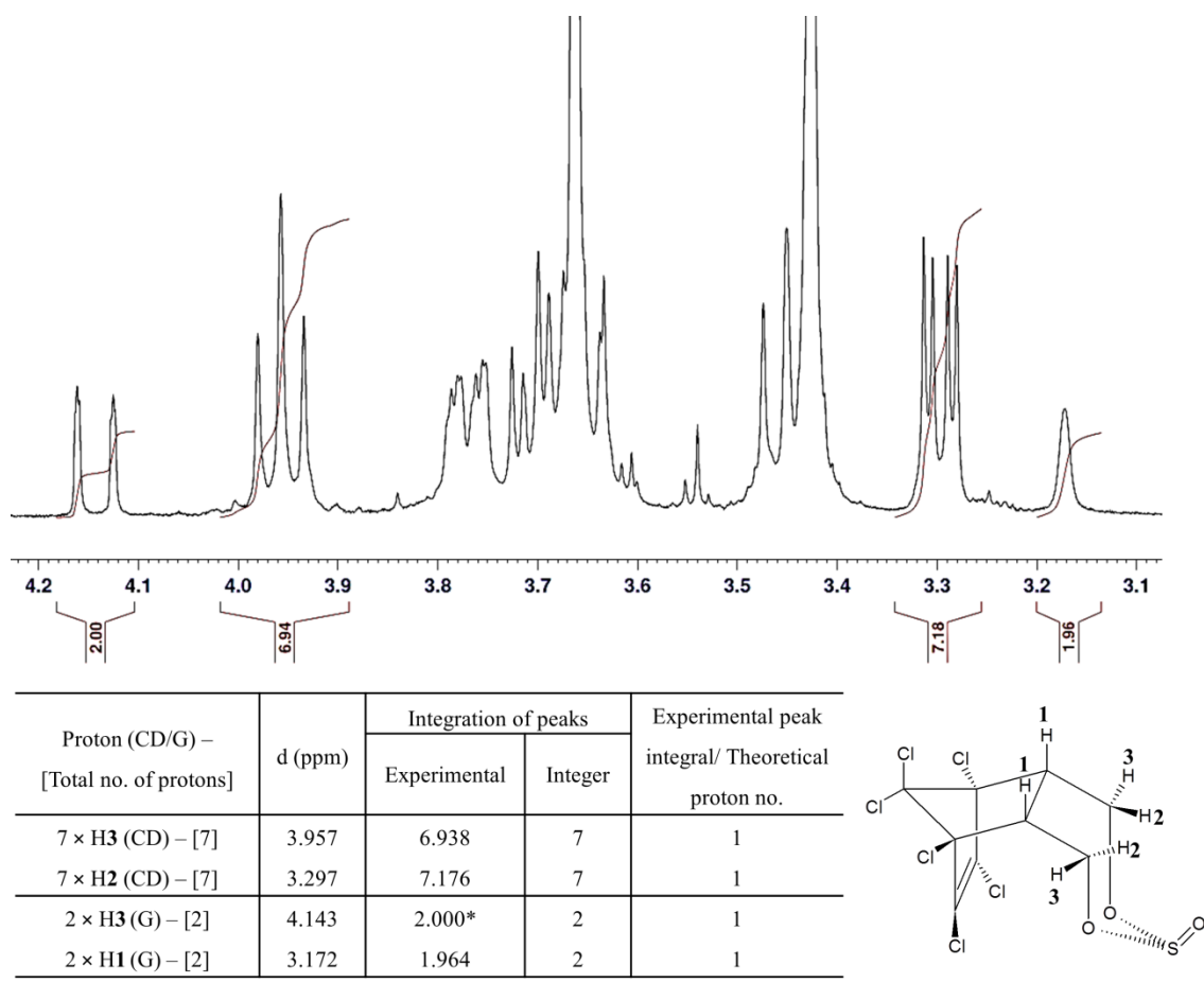
Figure S1. 1 H NMR spectra and tabulated results used to confirm the 1:1 host-guest ratio of the DIMEB·β-endosulfan complex.
