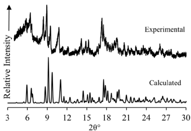
Figure S2. Calculated and experimental PXRD traces of the DIMEB·β-endosulfan complex.
