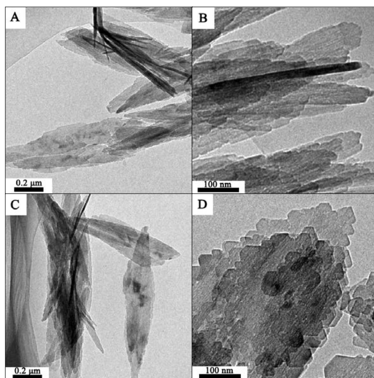
Figure S1. TEM images of as-synthesized AlOOH precursor for 6 h and its calcined product: (A, B) AlOOH , (C, D) Al 2 O 3 .
