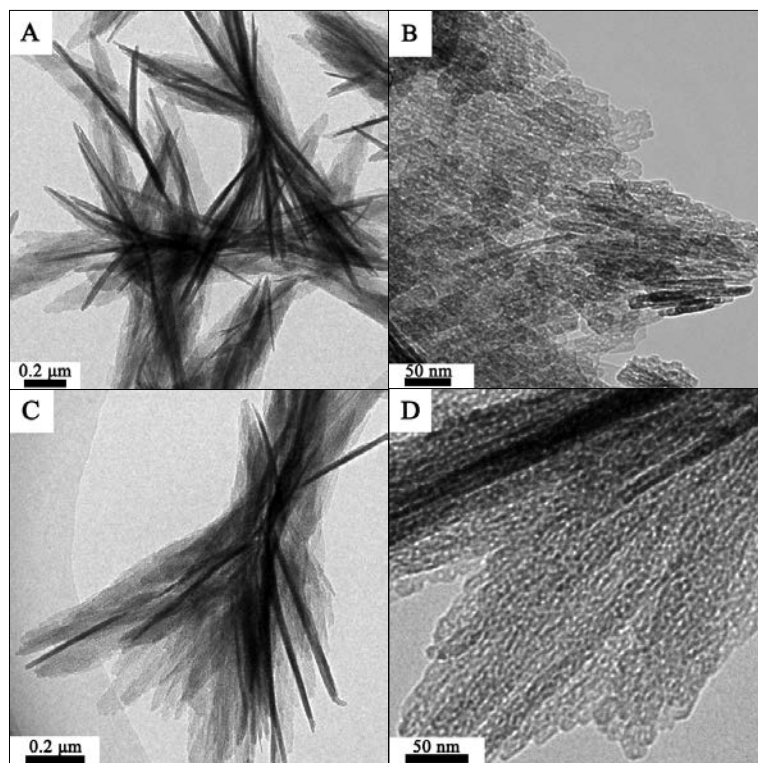
Figure S2. TEM images of as-synthesized AlOOH precursor for 48 h and its calcined product: (A, B) AlOOH , (C, D) Al 2 O 3 .
