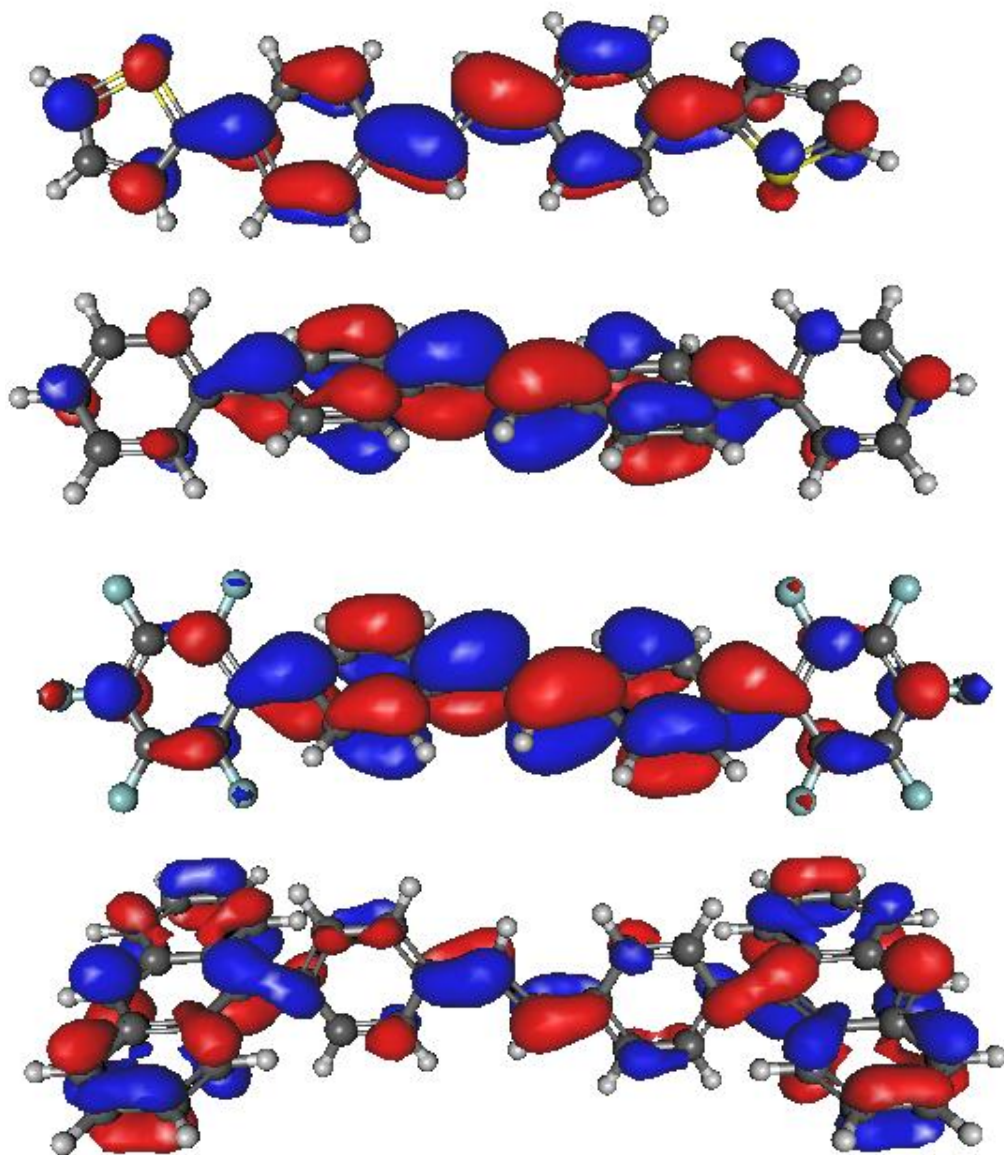
DFT-derived LUMO orbitals of the studied molecules.
