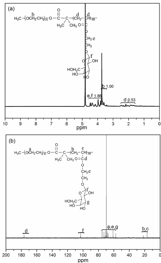
Fig. S2. (a) ^1\text{H} NMR and (b) ^{13}\text{C} NMR spectra of PEG- b -PAEG in \text{D}_2\text{O} .
