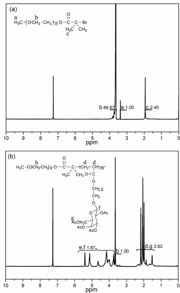
Fig. S1. ^1\text{H} NMR spectra of (a) PEG-Br and (b) PEG- b -PAEAcG in \text{CDCl}_3 .
