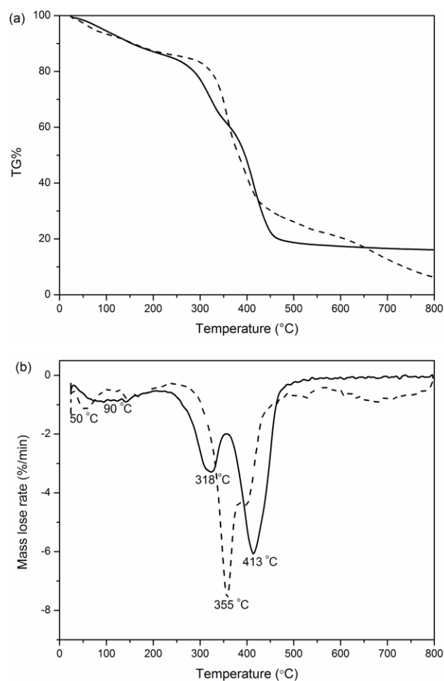
Fig. S4. Thermal analysis of PMAPBA/PEG- b -PAEG nanoparticles (dashed line) and the solid mixture of PMAPBA and PEG- b -PAEG (solid line): (a) TG; (b) DTG.
