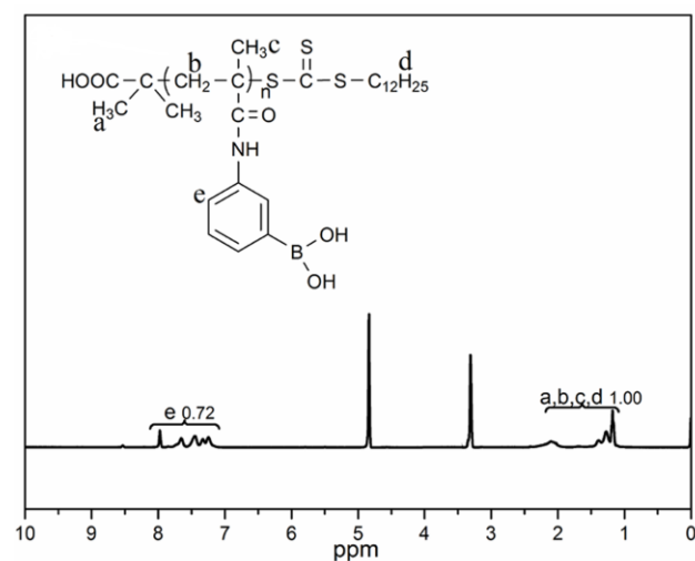
Fig. S3. ^1\text{H} NMR spectrum of PMAPBA in methanol- d_4 .
