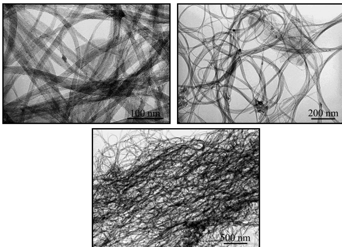
Figure S1. TEM images after the purification process with addition of oxygen in \text{Cl}_2/\text{N}_2 mixture applied on AD-SWNT; duration: 2 hours at 1100^\circ\text{C} .
