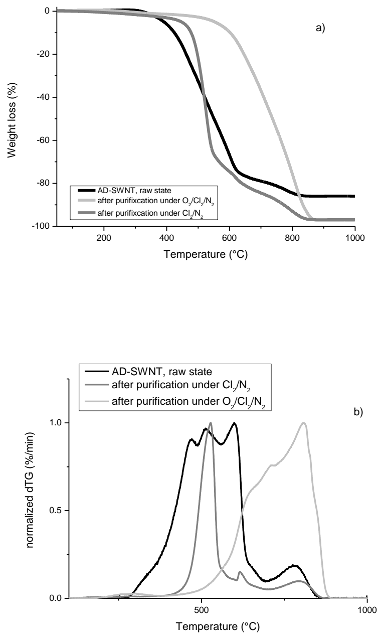
Figure S2. TGA (a) and dTG (b) profiles for AD-SWNT before and after purification under chlorine without and with oxygen; duration: 2 hours at 1100°C.
