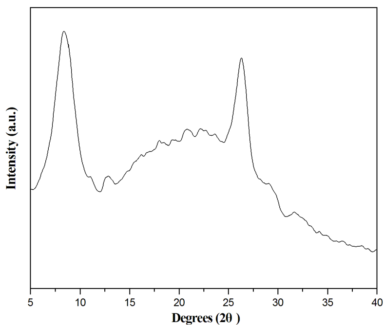
Fig. 2S. High angle X-ray diffraction pattern of the Cu-Salen-GO used for four cycles
