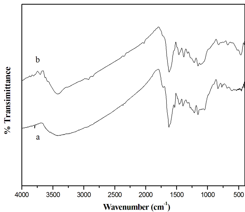
Fig. 1S. FT-IR spectrum of (a) the fresh catalyst Cu-Salen-GO and (b) the used catalyst Cu-Salen-GO for four cycles
