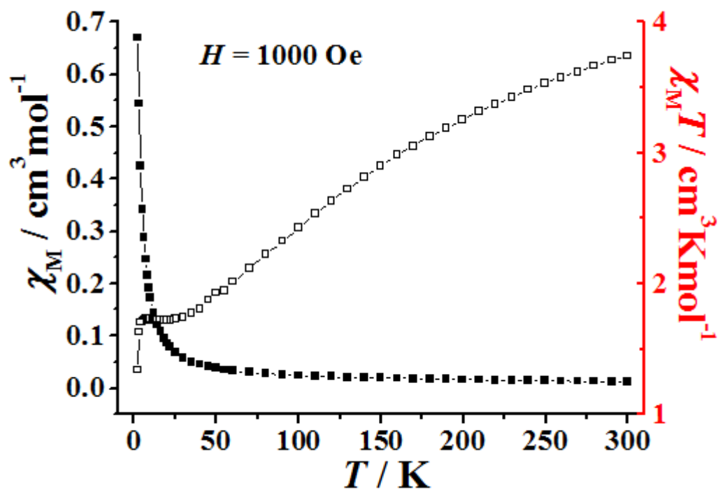
Fig. S3 The temperature dependence of the molar magnetic susceptibility \chi_M (■) and the product of the molar magnetic susceptibility and temperature \chi_M T (□) for 2 between 2 and 300 K.
