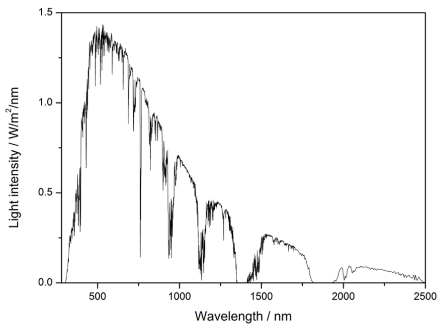
Figure S1 Solar radiation spectrum
