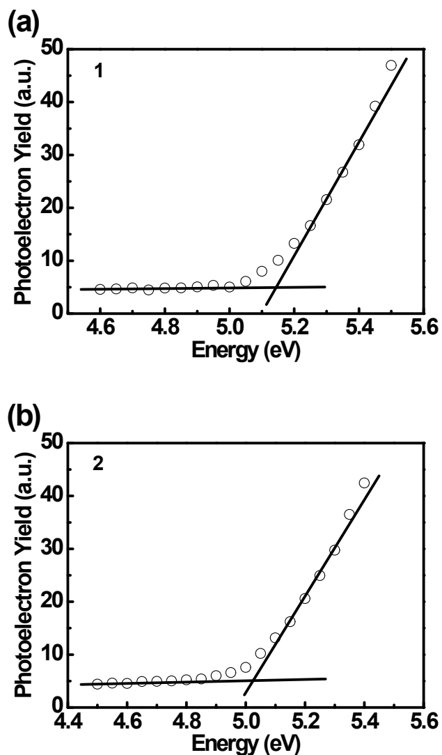
Figure S1. Photoelectron spectra of (a) compound 1 and (b) compound 2 thin films.
