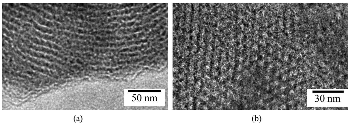
Figure SI1. HRTEM images of the original powders labelled OMPBN (a) and OMPSi/B/C/N (b).
