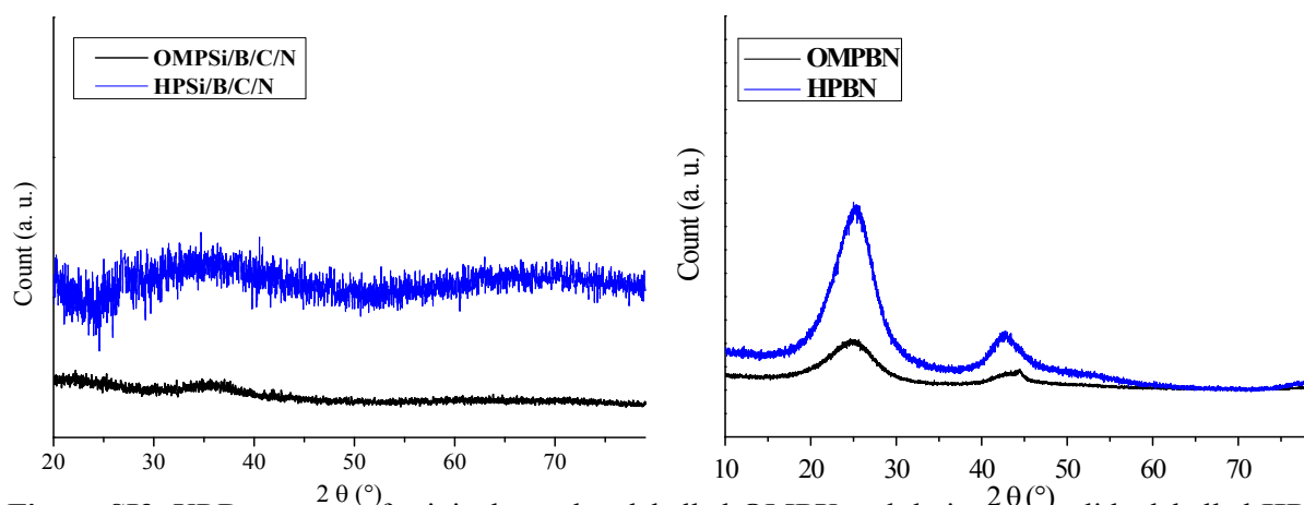
Figure SI3. XRD patterns of original powders labelled OMPX and derived monoliths labelled HPX (with X: BN, Si/B/C/N)
