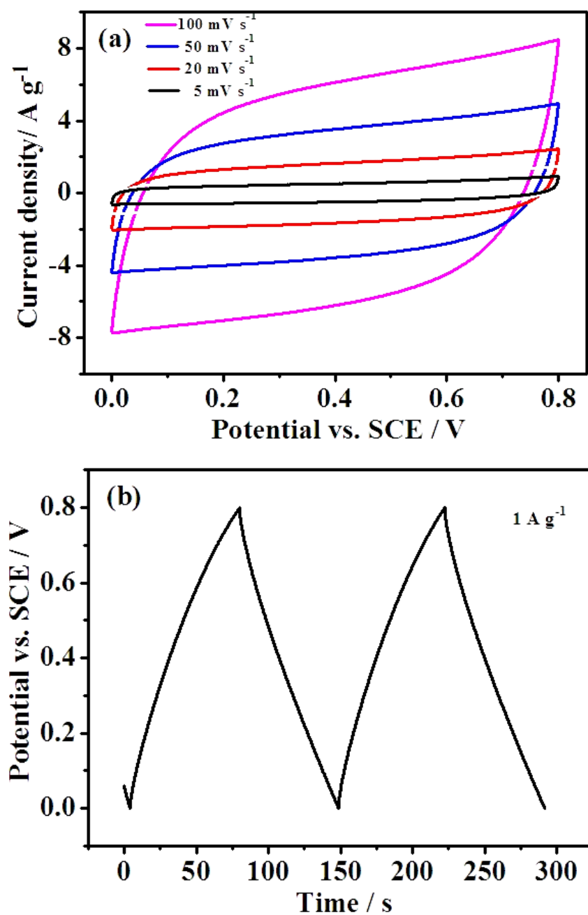
Fig.2 (a)CV and (b) charge-discharge curves obtained by the two-electrode supercapacitor cell.
