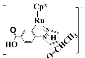
Ru-19
