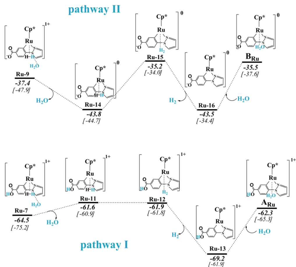
Figure S3. Detailed free energy profiles for another pathways beginning with intermediate Ru-7 (pathway I) and Ru-9 (pathway II), where waters are firstly dissociated. The values (italic numbers) are given in kcal/mol and enthalpies are listed in square brackets.
