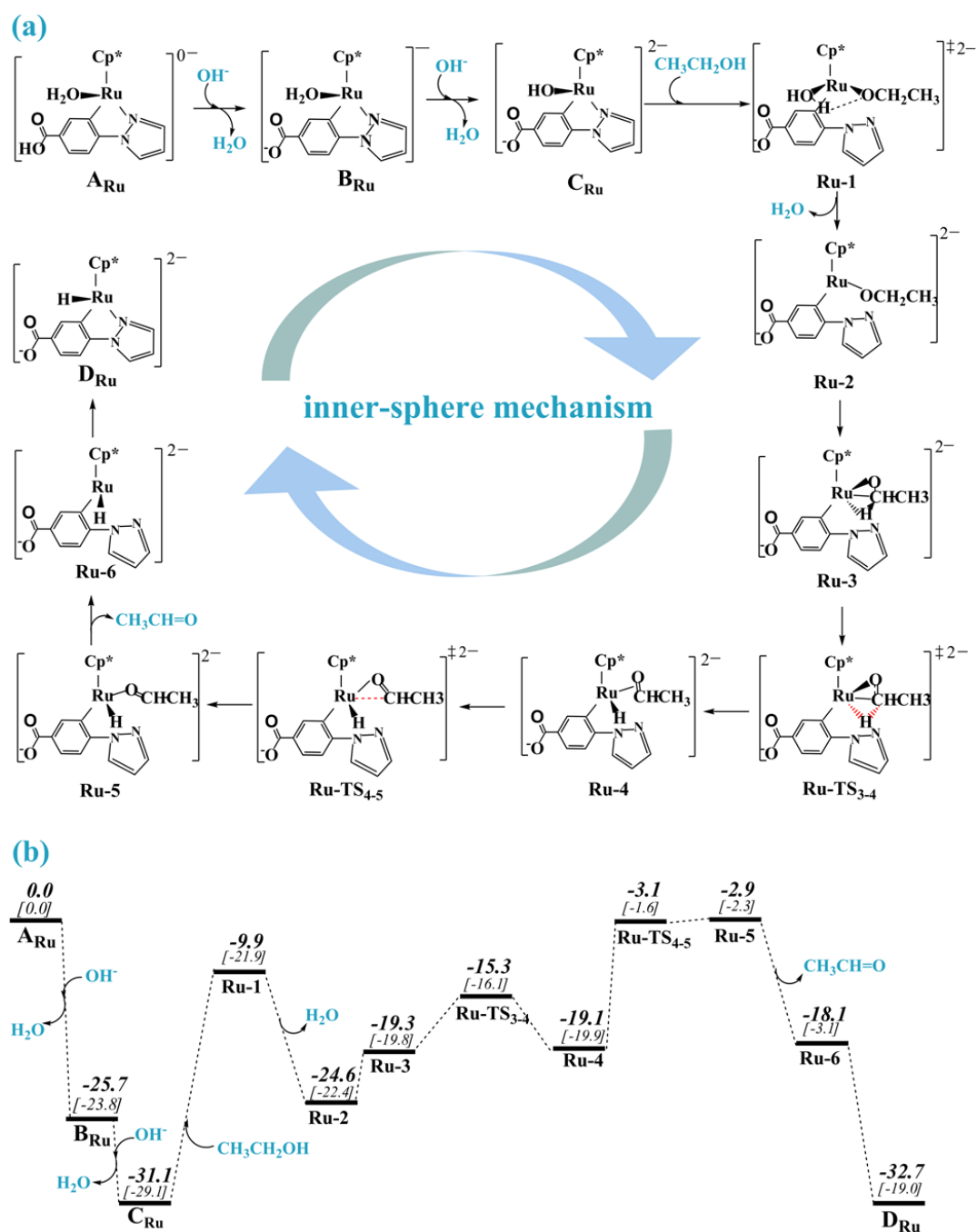
Figure S1. Detailed free energies profile of D_{Ru} formation through inner-sphere mechanism. The values (italic numbers) are given in kcal/mol and enthalpies are listed in square brackets.
