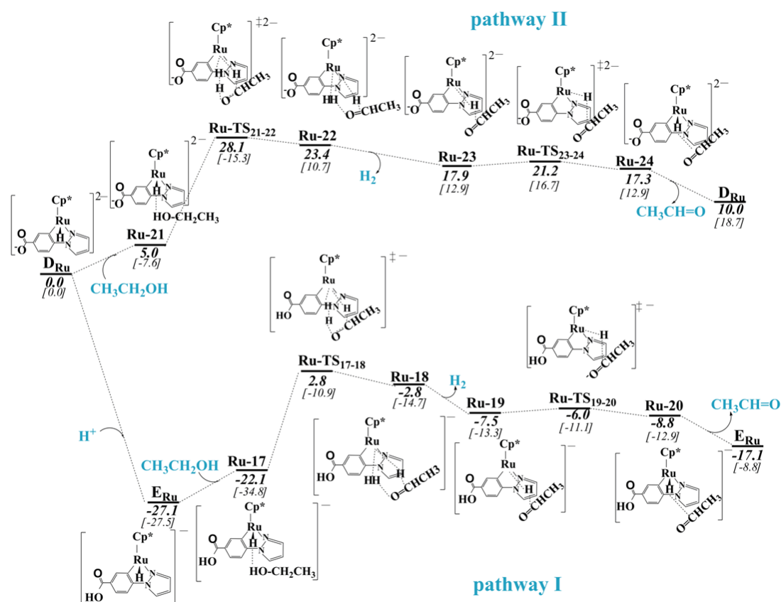
Figure S4. Detailed energy profiles of the H 2 formation based on the complex D Ru and the ethanol, including the free energies and enthalpies (in brackets) in M06/BSII (SMD, water) level (in kcal/mol).
