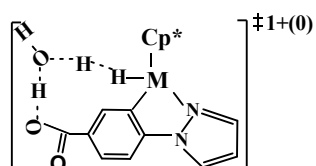
H 2 O-TS 1-2
