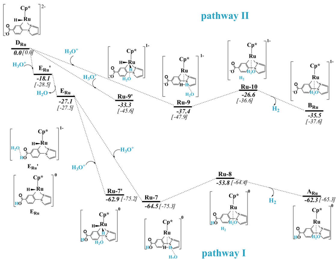
Figure S2. Detailed energy profiles of the H 2 formation based on the complex D Ru and the proton, including the free energies and enthalpies (in brackets) in M06/BSII (SMD, water) level (in kcal/mol).
