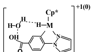
H 2 O-1
