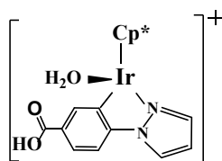
\text{A}_{\text{Ir}}
