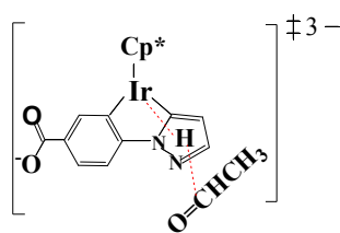
3-TS 3.4
