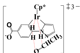
3-TS 1-2
