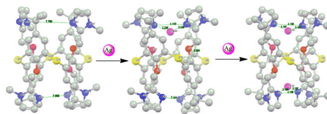
Fig. 7. Geometry-optimized (ball-and-stick) structures of: Left: 4 ; Middle: 1:1 complex of \text{4} \rightarrow \text{Ag}^+ and Right: 2:1 complex of \text{Ag}^+ \leftarrow \text{4} \rightarrow \text{Ag}^+ . Colour code: \text{Ag}^+ = magenta, imidazole nitrogen = blue, sulphur = yellow and oxygen atom = red. Hydrogen atoms have been omitted for clarity.
