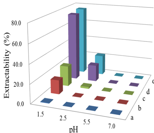
Fig. 9. Extraction percentages of dichromate anion with 1,3-alternate-4 and reference 6 at pH 1.5–7.0 (H 2 O/CH 2 Cl 2 :10/10 (v/v); K 2 Cr 2 O 7 = 1 × 10 -4 M; ligand: (a) reference 6 , 4.0 × 10 -4 M; (b) 1,3-alternate-4 , 0.5 × 10 -4 M; (c) 1,3-alternate-4 , 1.0 × 10 -4 M; (d) 1,3-alternate-4 , 2.0 × 10 -4 M; (e) 1,3-alternate-4 , 4.0 × 10 -4 M, 1 h at 25 °C).
