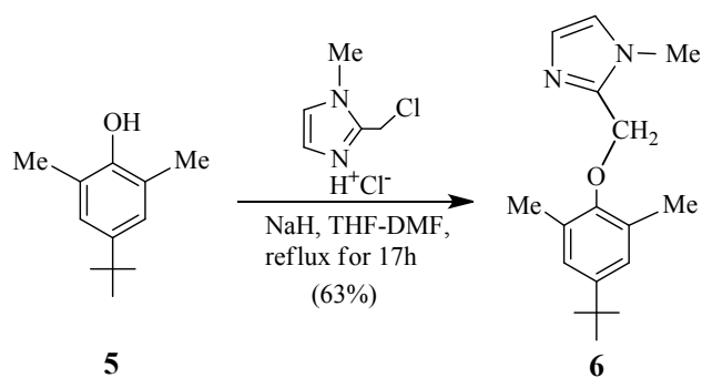
Scheme 2 Synthesis of the reference compound 6 .
