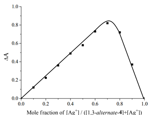
Fig. 5 Job's plot for complexation of 1,3-alternate-4 with \text{Ag}^+ ion.
