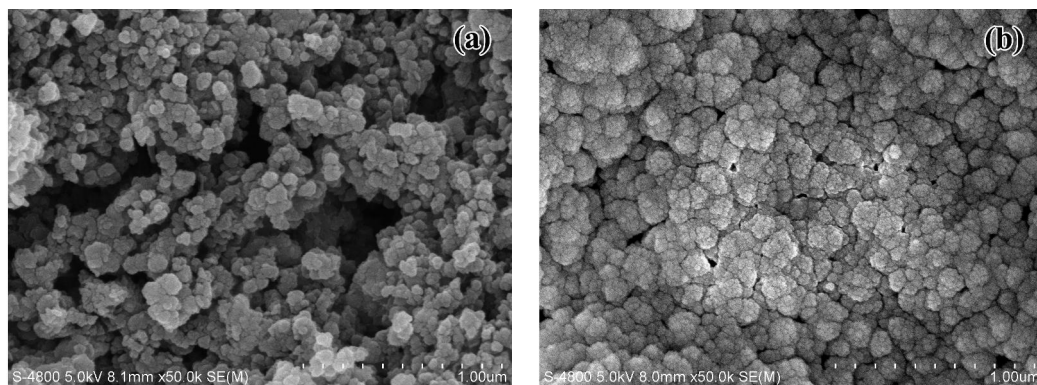
Fig. S1. Field-emission scanning electron microscope images of (a) fresh TiO 2 /MoS 2 electrode, (b) TiO 2 /MoS 2 electrode after 100 cycles between at a current density of 100 mA g -1
