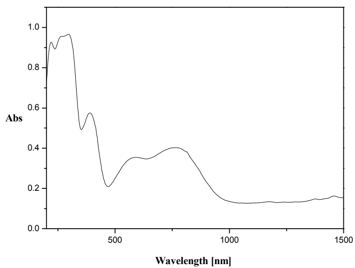
Figure S5. The UV-Vis spectra for complex 2
