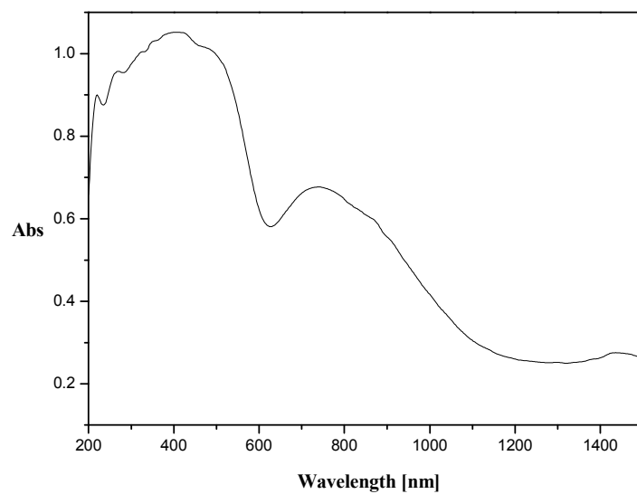
Figure S6. The UV-Vis spectra for complex 3
