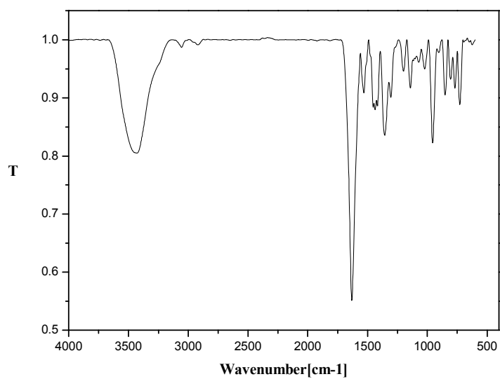
Figure S3. The IR spectra of complex 3
