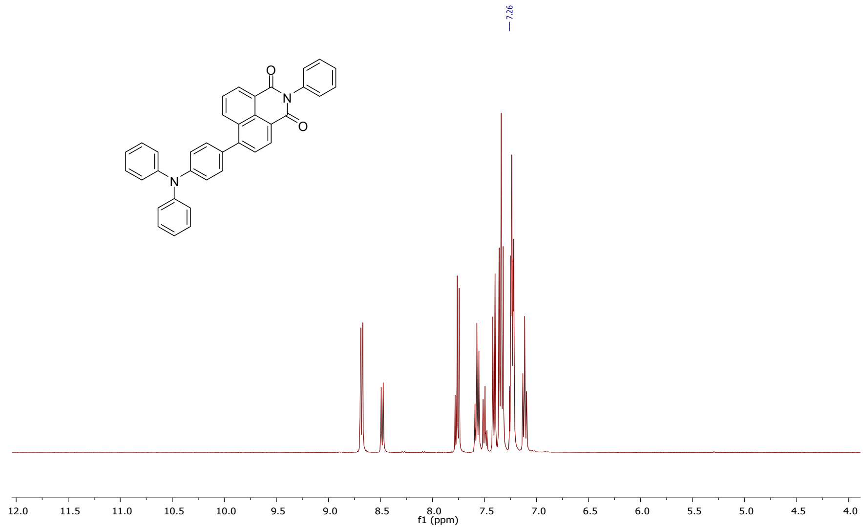
Fig. S3 1 H-NMR of TPN1 in CDCl 3
