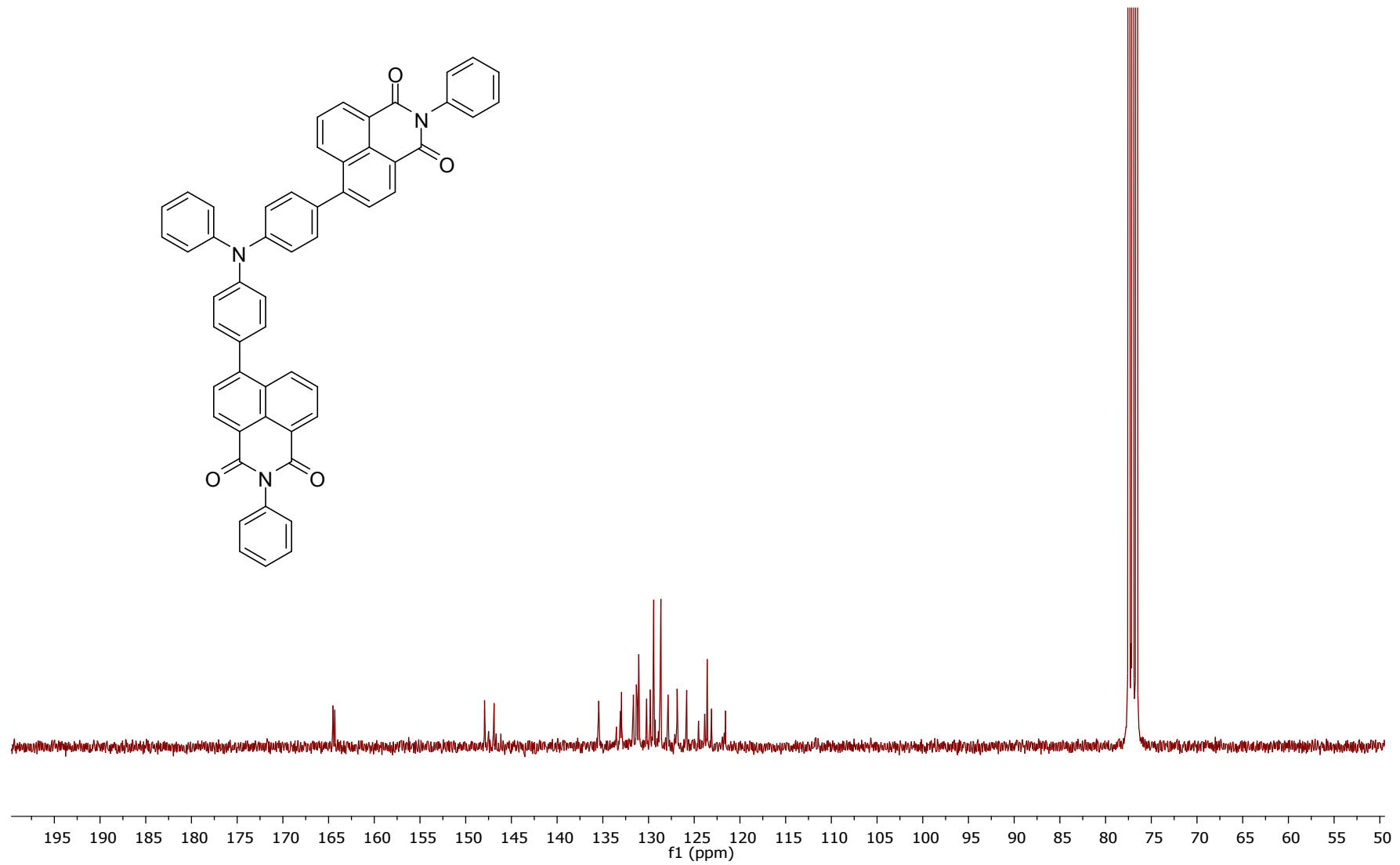
Fig. S6 13 C-NMR of TPN2 in CDCl 3
