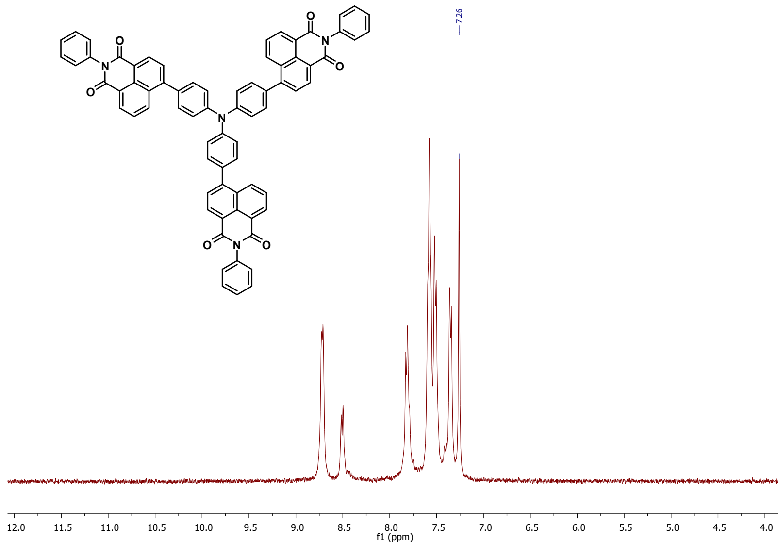
Fig. S7 1 H-NMR of TPN3 in CDCl 3
