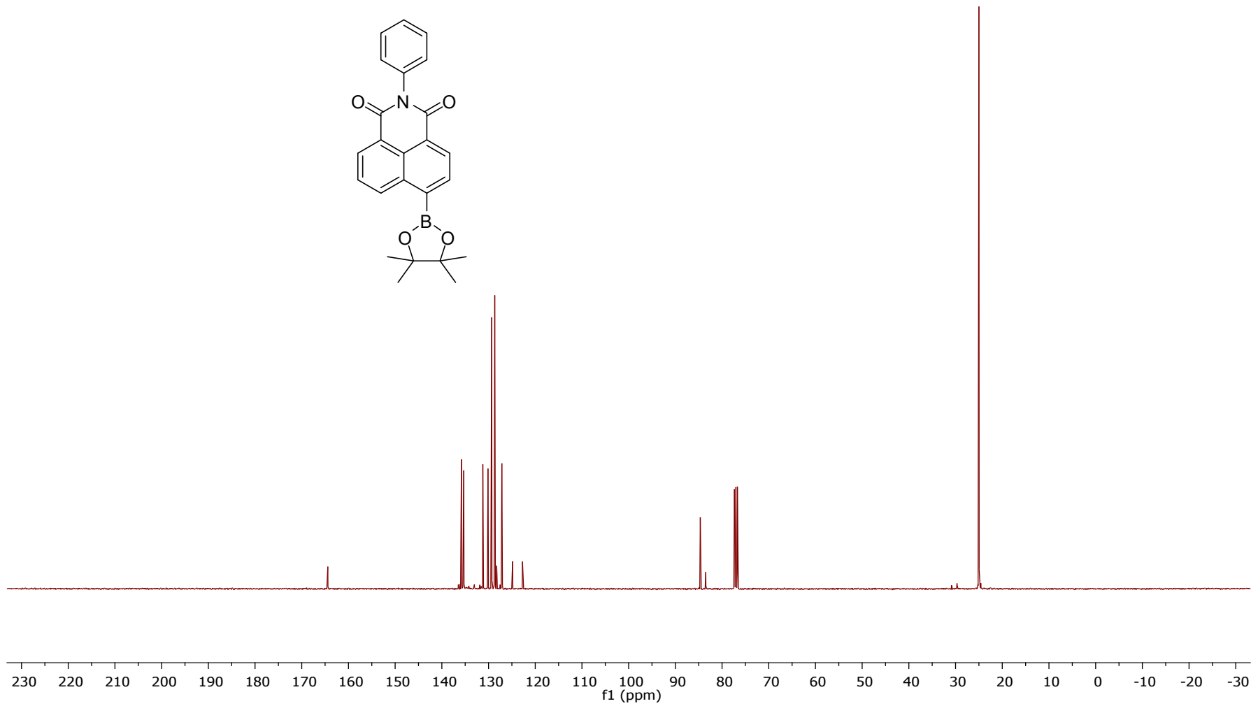
Fig. S2 ^{13}\text{C} -NMR of A in \text{CDCl}_3
