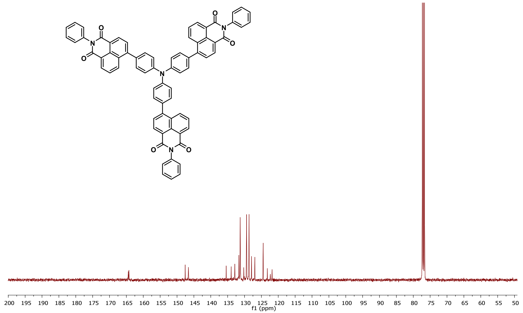
Fig. S8 13 C-NMR of TPN3 in CDCl 3
