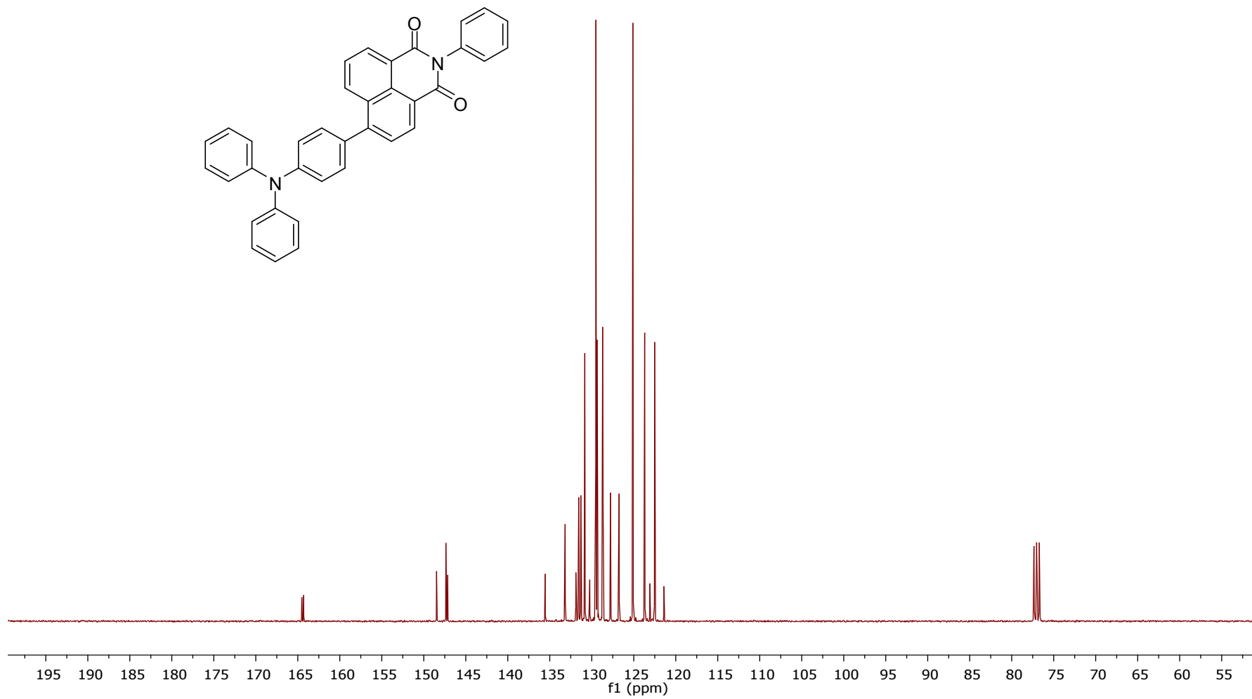
Fig. S4 ^{13}\text{C} -NMR of TPN1 in \text{CDCl}_3
