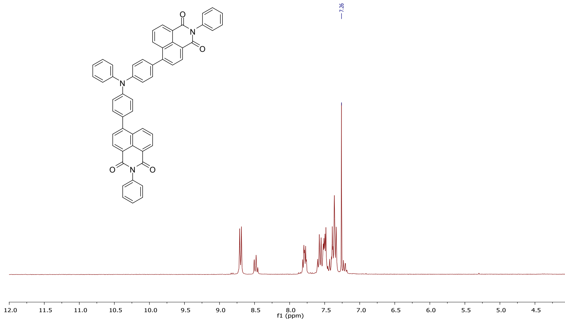
Fig. S5 1 H-NMR of TPN2 in CDCl 3
