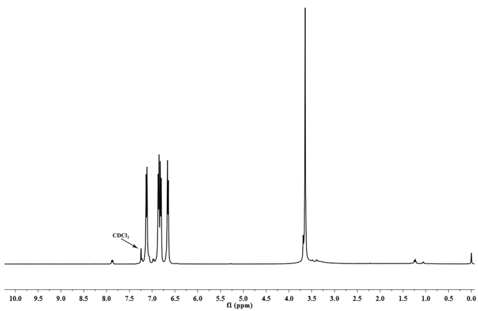
Figure S2 ^1\text{H-NMR} spectrum of OAPS
