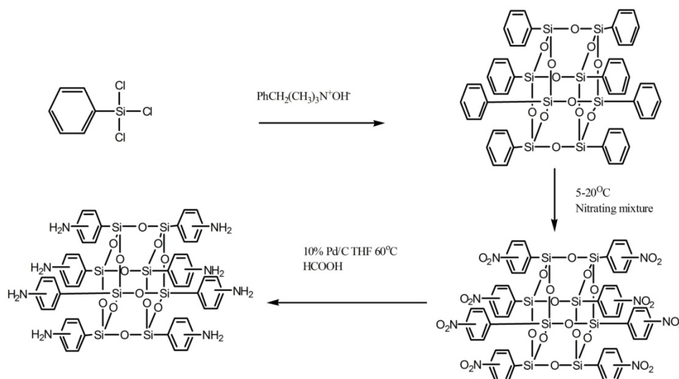
Scheme S1: Synthesis of amine functionalized POSS
