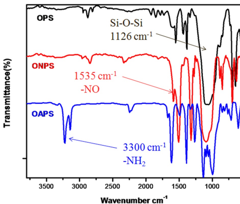
Figure S1 FT-IR spectra of OPS, ONPS and OAPS
