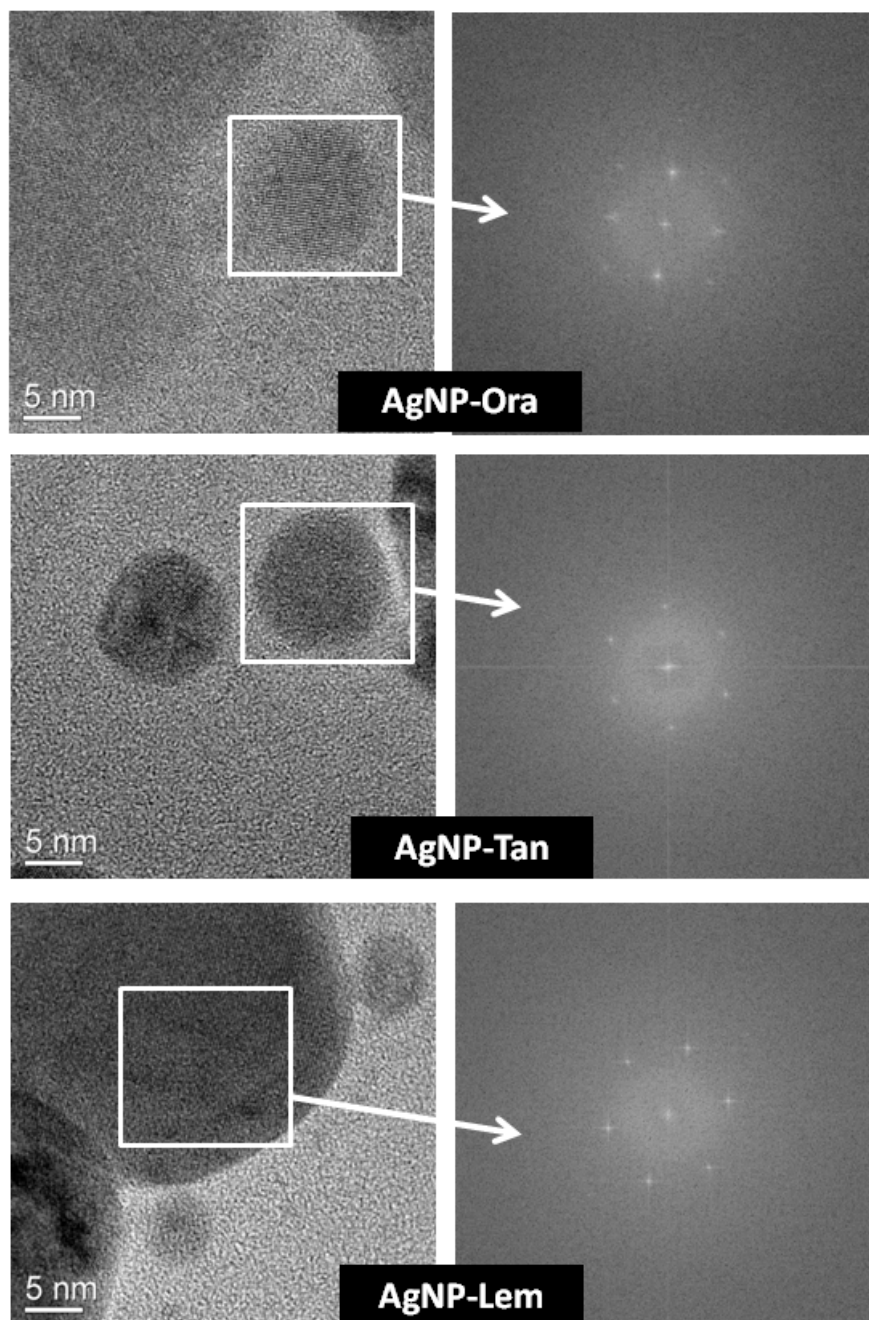
Figure SM2. HRTEM images of the AgNP-Ora, AgNP-Tan, and AgNP-Lem.
