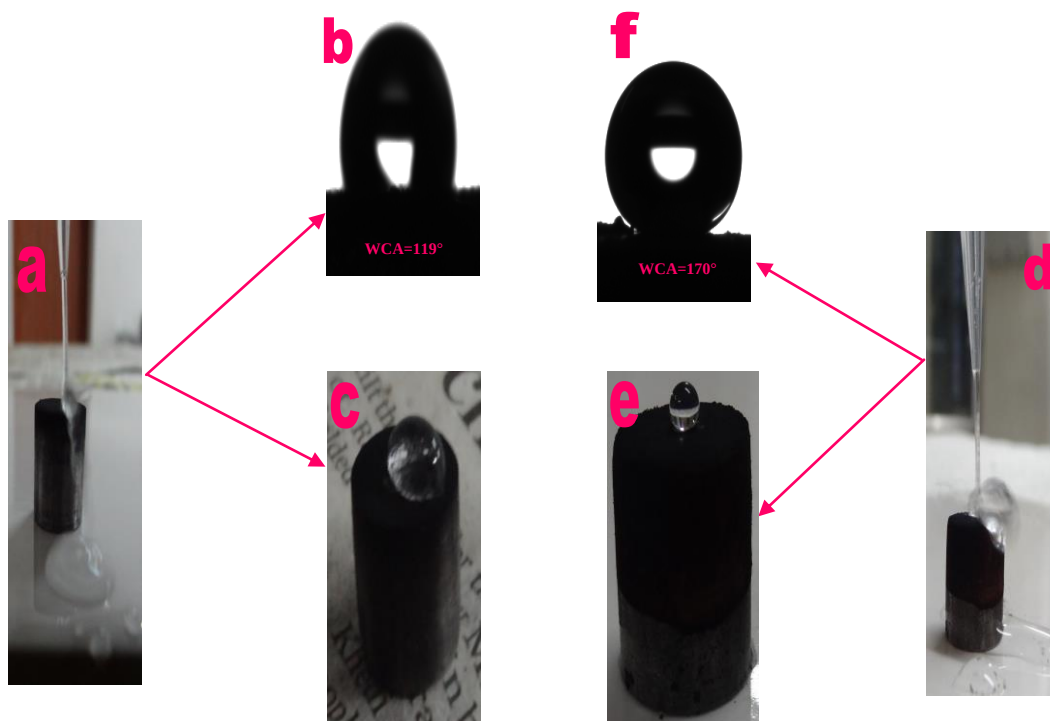
Fig. S3 Schematic diagram of water-flow impact test (a,d), water contact angles (b,f) and photographs of water droplet on ST/Al and ST/Cu/Al surfaces (c,e) respectively.
