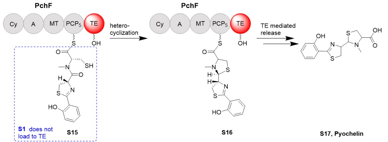
Fig. S4: Terminal ring-specific release of pyochelin precursor is supported by PchF TE's substrate specificity
