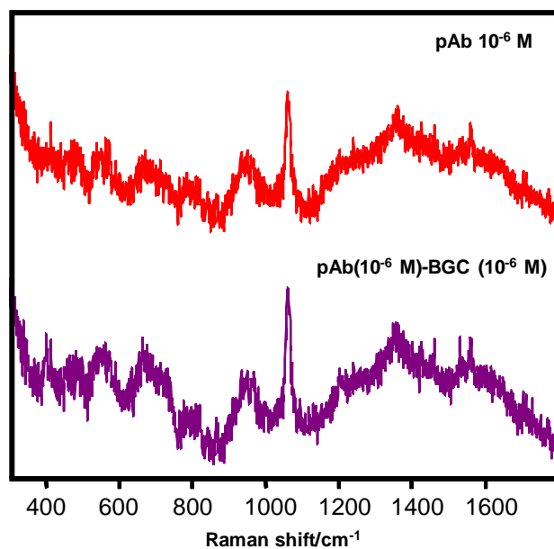
Figure S1. SERS spectra of polyclonal antibodies on CNT@Ag before and after exposure to BCG.
