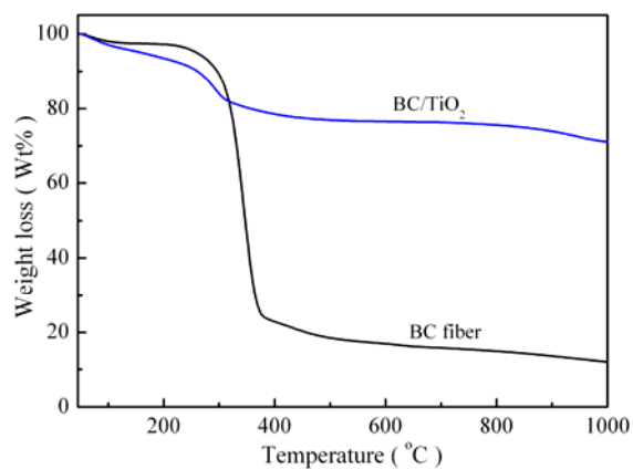
Figure S1. Thermogravimetric analysis curves for BC nanofibers and BC/TiO 2 hybrid nanofibers.
