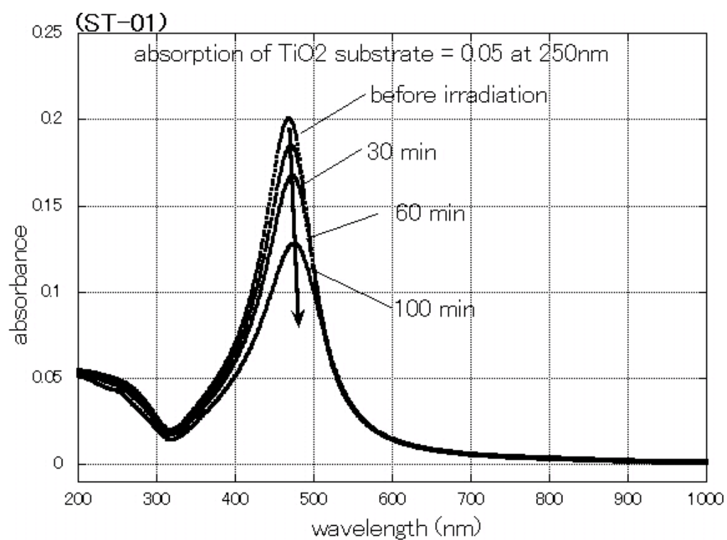
Suppl._1 Spectrum change of Ag nanosheet deposited on ST-01TiO 2 particles (1min adsorption) by UV irradiation.
