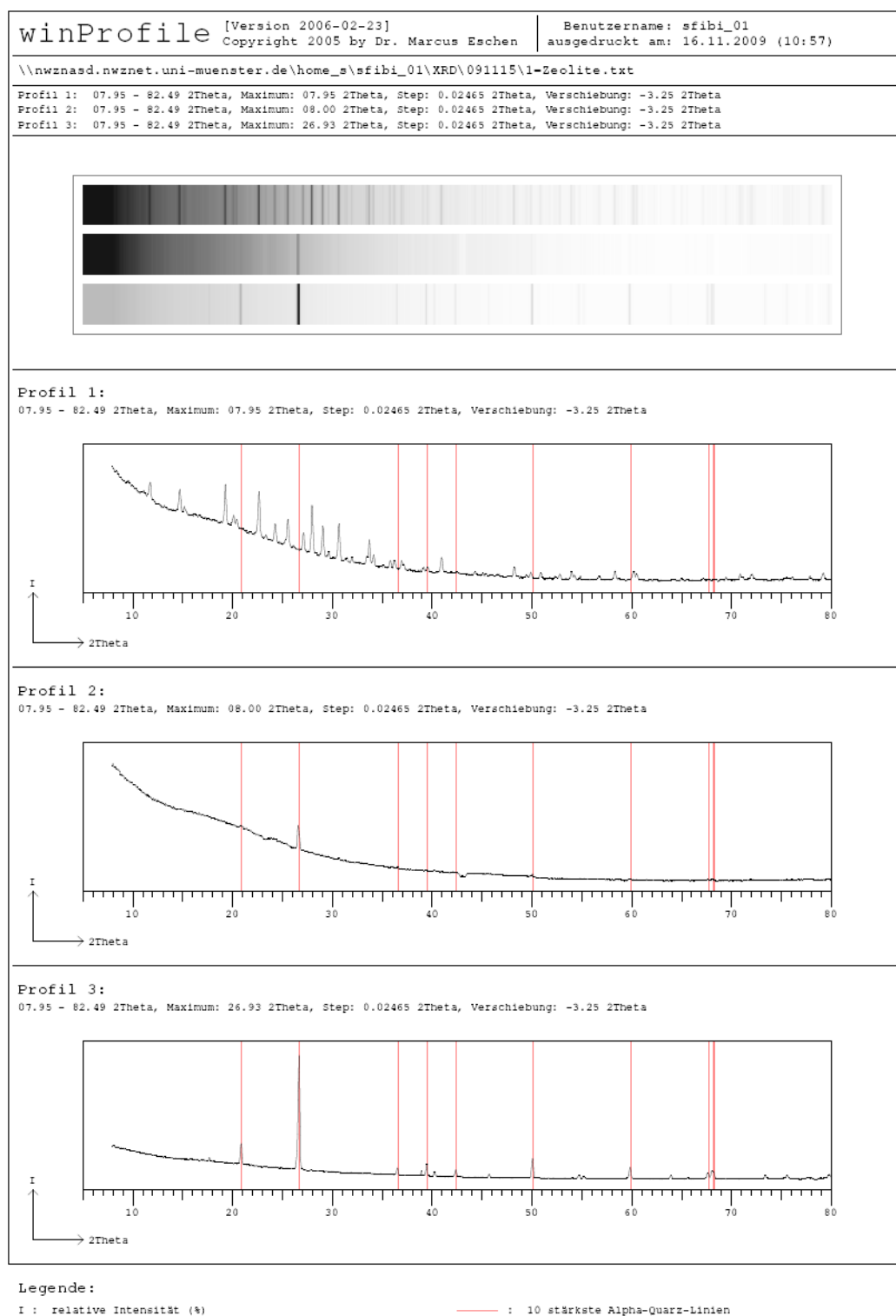
Figure S5. X-ray powder diffraction pattern (taken in transmission mode) for zeolite L crystals.
