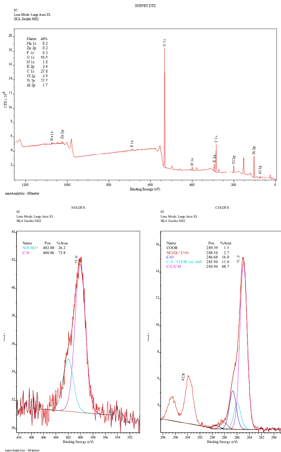
Figure. S1. XPS spectrum of amino functionalized SAM of zeolite.
