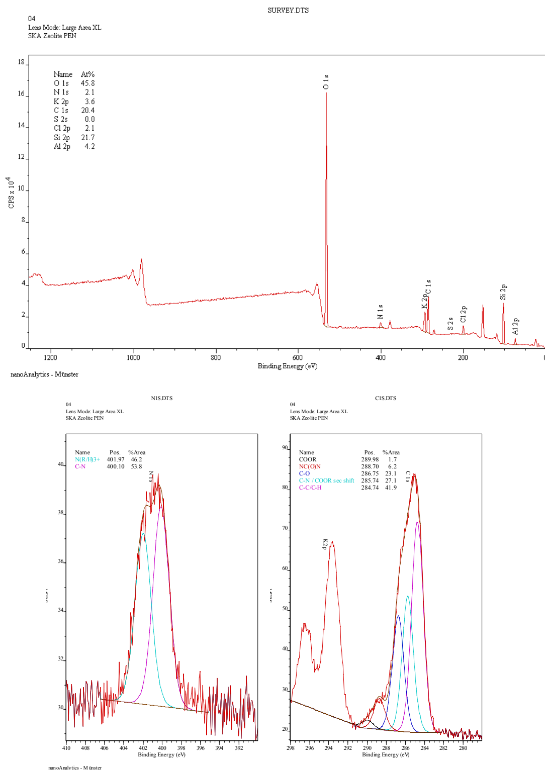
Figure. S4. XPS spectrum of of PEN functionalized SAM of zeolite.
