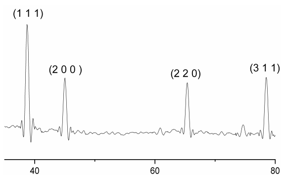
Fig. 3: XRD spectrum of Al/PMMA (1:1) composite
