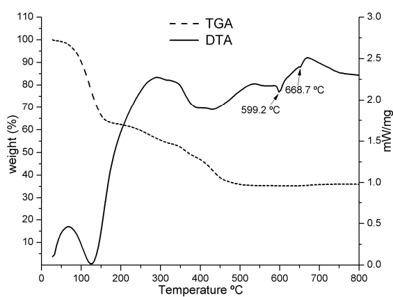
Fig. 2: TG-DTA curves of Al/PVP composite after removing lithium chloride
