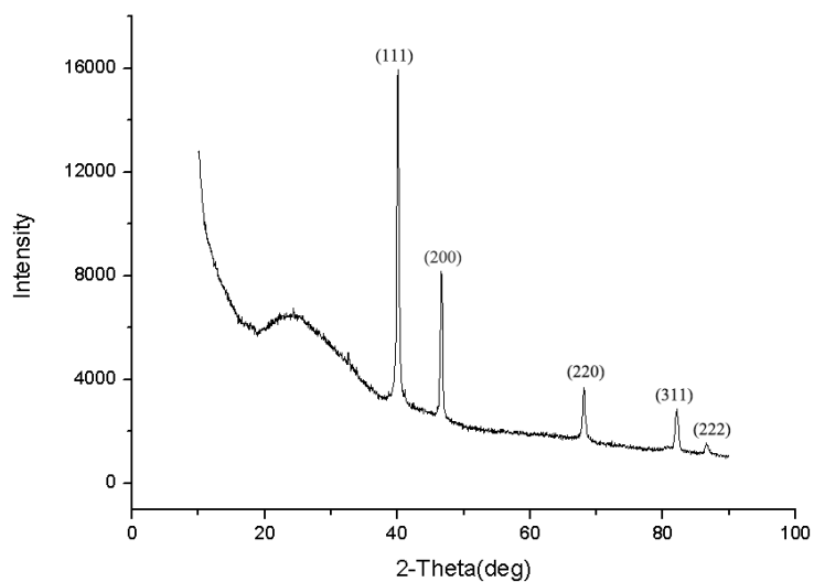
Fig.S2 XRD pattern of the palladium seeds.
