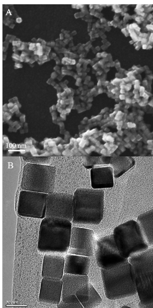
Fig.S1 SEM (A) and TEM (B) images of the palladium seeds.
