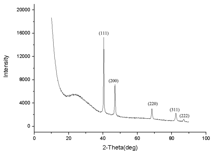
Fig.S4 XRD pattern of the palladium nanocrystals obtained in the presence of 10 \mu M KSCN at 60°C.
