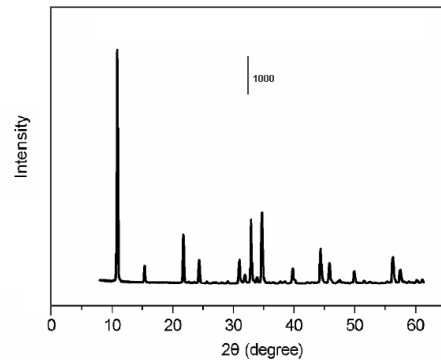
Figure S2. XRD pattern of structures of the nanobelts of sample 1.
