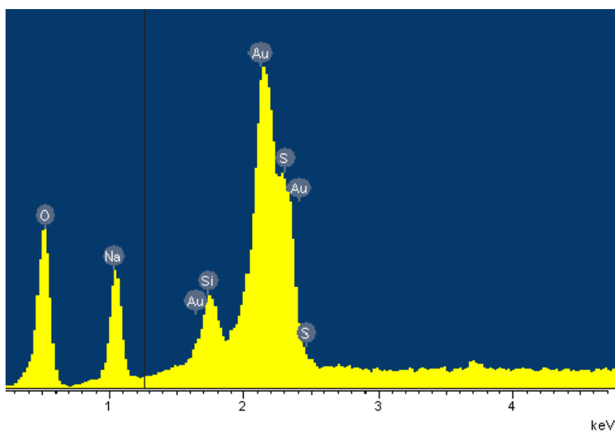
Figure S1. EDS of structures of the nanobelts of sample 1.
