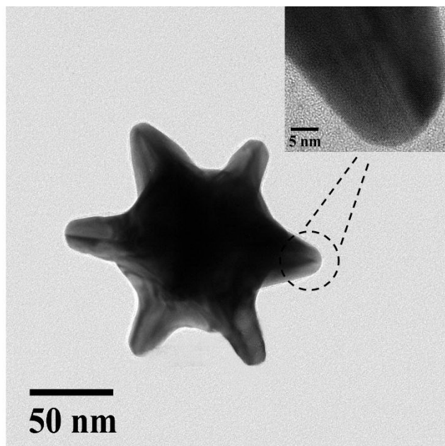
Fig. S1. The high-resolution TEM (HRTEM) image of a well-formed \text{Fe}_3\text{O}_4@\text{GNS}
