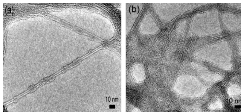
Figure S2. TEM images of the suspension of DWNTs-SWNTs mixture.
