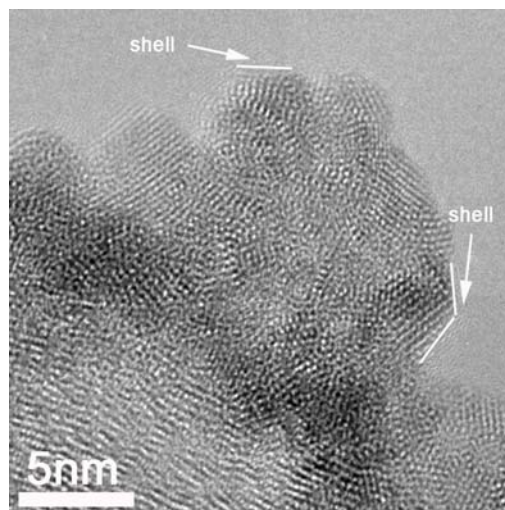
Fig. S1 Magnified HRTEM image of \text{CoSn}_3 -MWCNTs nanohybrids.
