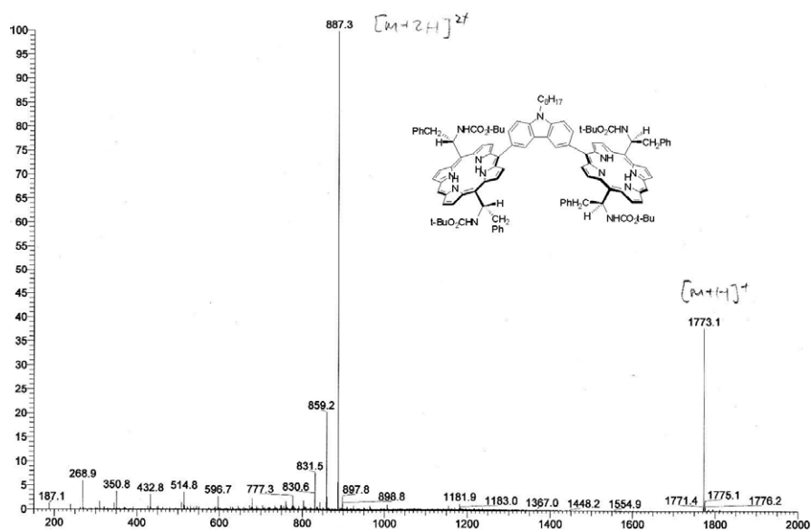
Fig. S2. HR-ESI-MS spectrum of free base diporphyrin after removal of Zn in (R)-1. (S)-Isomer shows the same spectrum.
