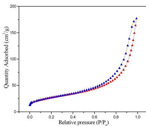
Fig. S2 Nitrogen adsorption/desorption isotherm of graphene nanoplate-MnO 2 composite obtained at 3 h.
