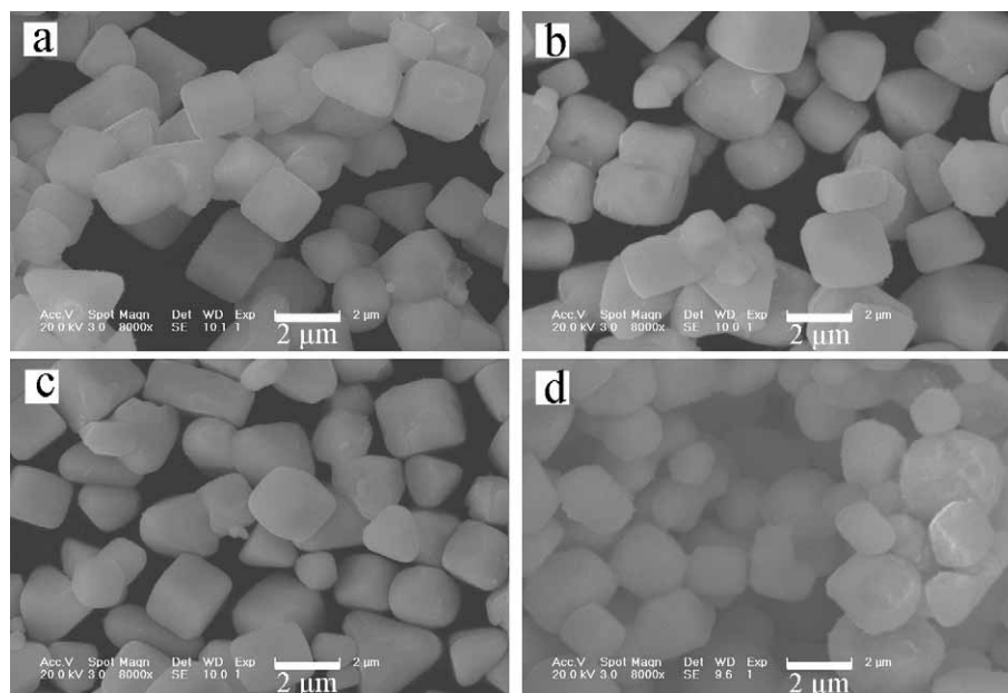
Figure. S2 The typical SEM of the as-prepared AgCl with different addition of AgNO 3 : 0.091 g (a), 0.146 g (b), 0.182 g (c) and 0.270 g (d), respectively.
