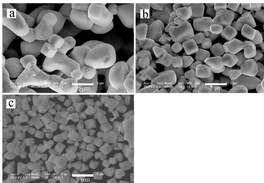
Figure. S1 The typical SEM of the as-prepared AgCl with different addition amount of PVP: 0 g (a), 0.356 g (b) and 0.713 g (c), respectively.
