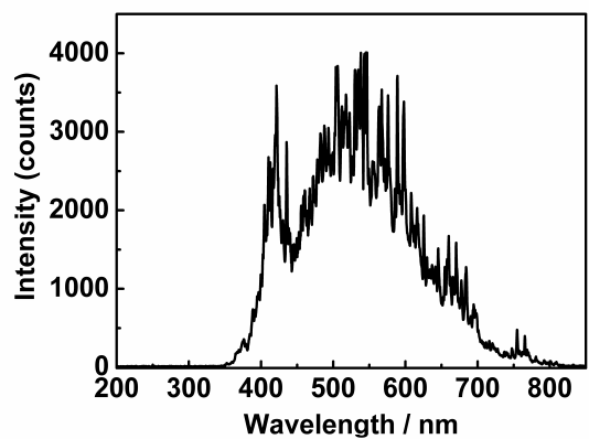
Figure S1. The optical spectrum of the 150 W halogen lamp used in the photocatalytic reaction.
