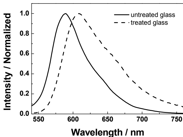
Figure S1 Spectra of PBI 1 monomers spin-coated from MCH solution ( c = 10^{-8} M, the diluted solution was kept for two days at room temperature to ensure dissociation into monomers) onto untreated glass substrate (solid line) and treated substrate (dash line).
