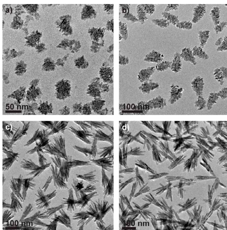
Figure S1. TEM images of the zinc oxide nanostructures at reaction times of a) 2 min, b) 5 min, c) 6 h and 12 h.
