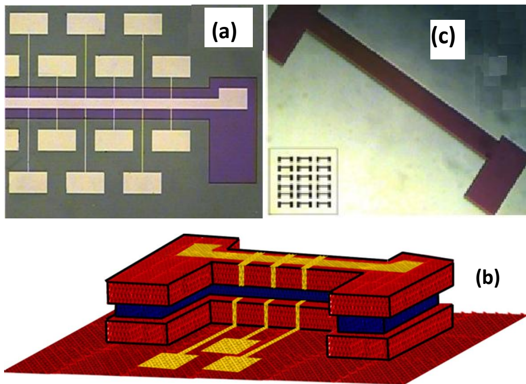
Figure S1 (a) Optical microscope image of an array of mesa nanojunctions and (b) Three dimensional schematic presentation of an array consisting of few nanojunctions. (c) Optical microscope image of a single mesa structure just after nanogap formation, inset shows the mask pattern.
