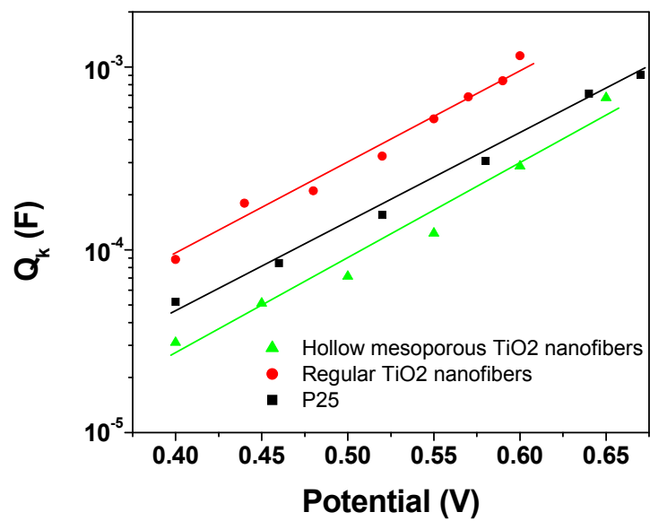
Fig 3. Chemical capacitance Q_k
