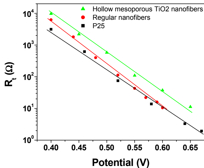
Fig 1. Electron transport resistance R_t
