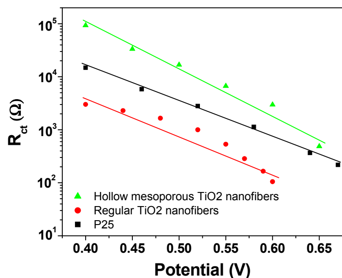
Fig 2. Electron recombination resistance R_{ct}
