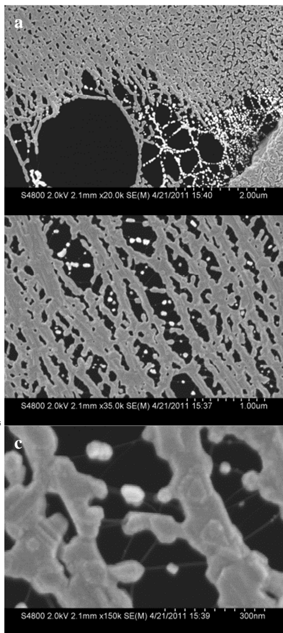
Fig S1. SEM images of h -CdSe-SWCNT with 5-min CVD.
