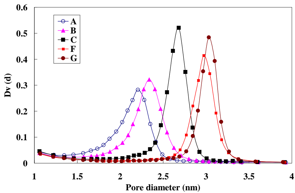
Figure S1. Pore size distribution for A,B,C,F and G samples
