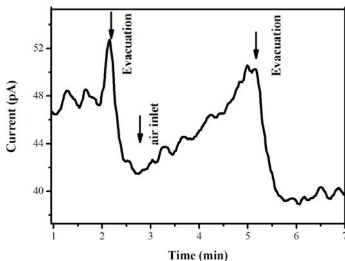
Figure S4. The variation of conductance of a single CdTe NR upon the switch of ambient between air and vacuum of 2 \times 10^{-1} torr.
