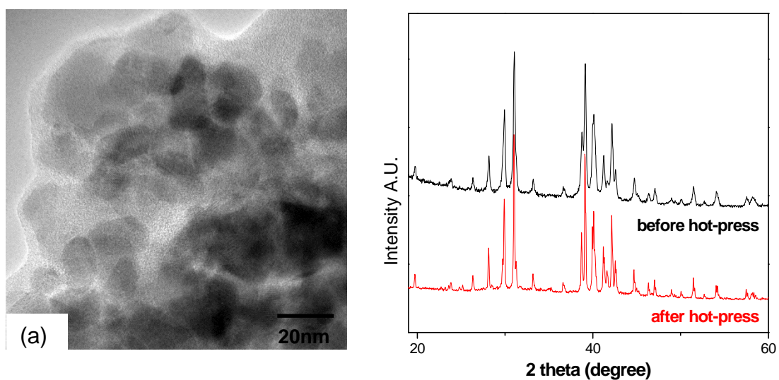
Figure S2 (a) TEM image and (b) XRD pattern of 15-nm \text{Ag}_2\text{Te} particles after hot-pressed at 673 K
