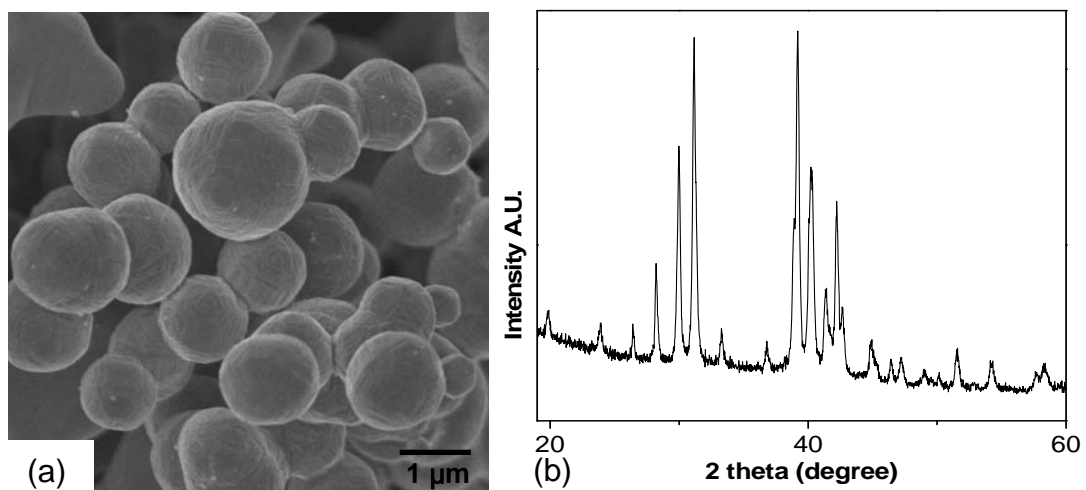
Figure S1 (a) SEM image and (b) XRD pattern of \text{Ag}_2\text{Te} particles synthesized without dodecanethiol at 443K for 10min
