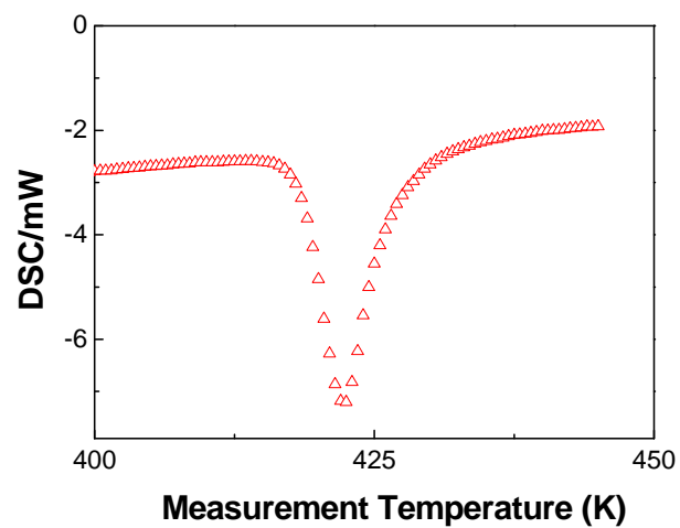
Figure S3 Temperature dependent DSC result of 15-nm Ag 2 Te nanoparticles
