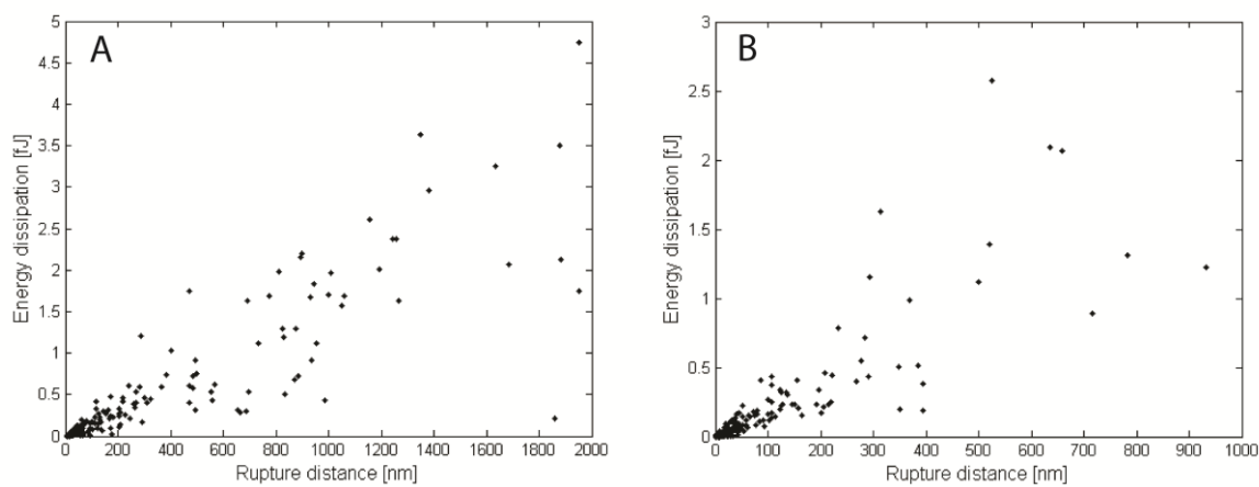
Figure S1. Correlation between the amount of dissipated energy and the final detachment distance for the case of interaction between a heavily demineralized gastrolith probe (A) and a native gastrolith sample and between a CaCO 3 probe and a native gastrolith sample (B), respectively.
