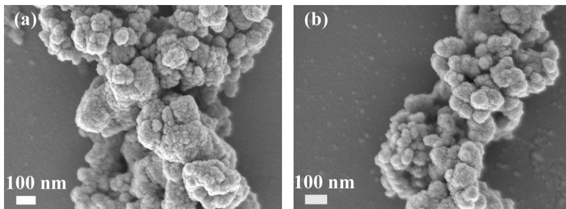
Fig. S2 The SEM images of the products with different usages of glucose: (a) 1.5 g and (b) 2.5 g.
