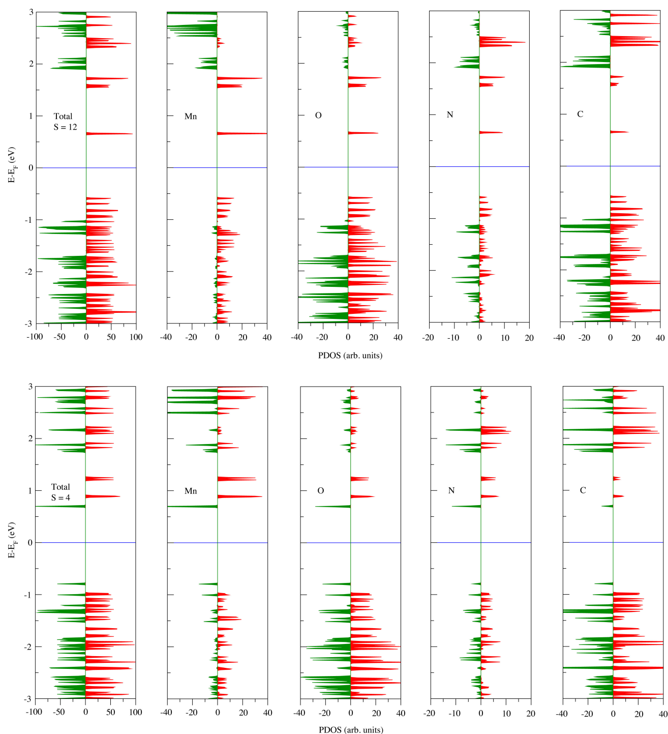
Figure S2. Total and projected density of states (red and green curves indicate alpha and beta spin states, respectively) for the S = 12 (above) and S = 4 (below) of the [\text{Mn}_6\text{O}_2(\text{Me-sao})_6\{\text{O}_2\text{CPh}(\text{SH})\}_2(\text{MeOH})_6] model complex.
