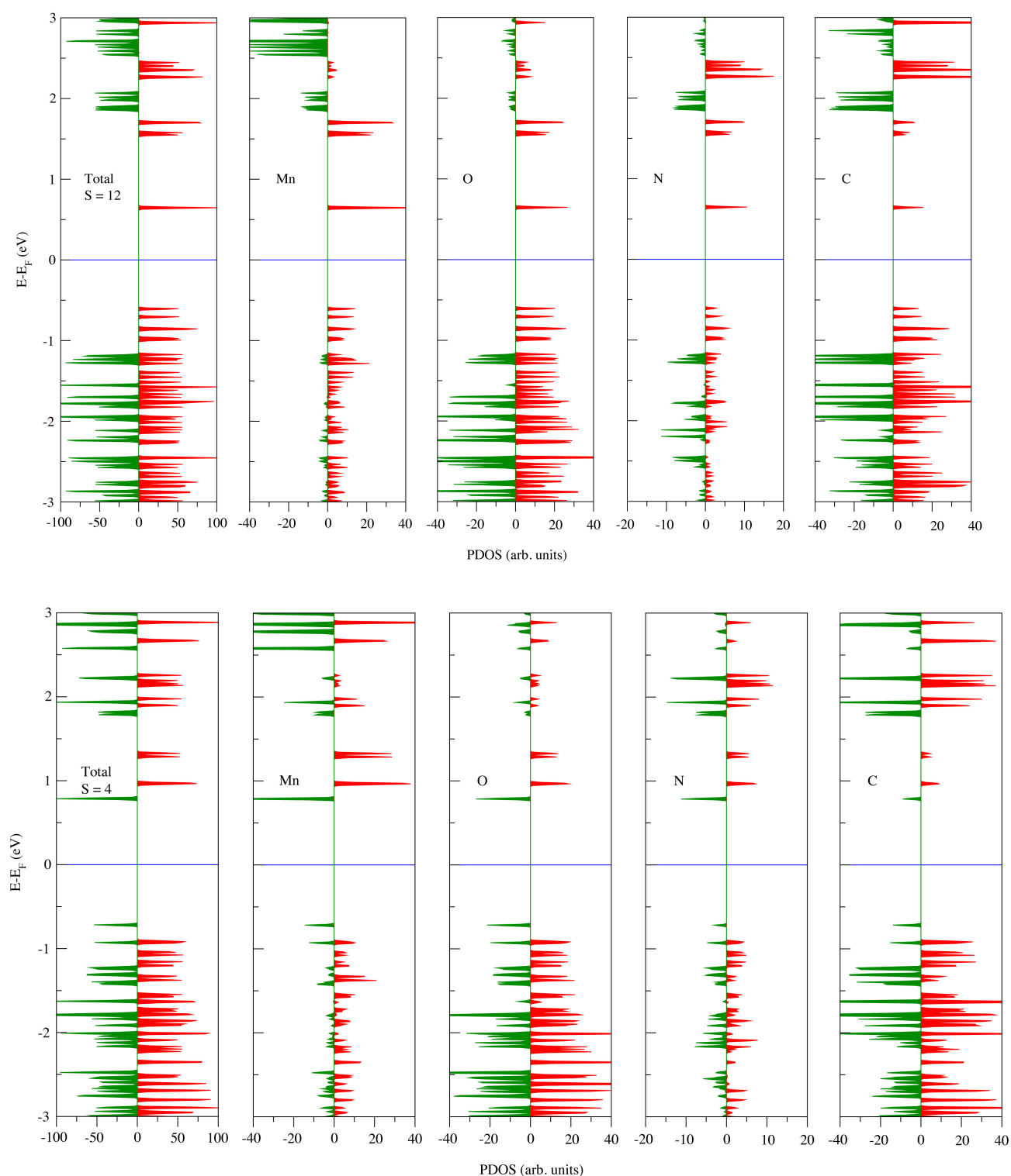
Figure S1. Total and projected density of states (red and green curves indicate alpha and beta spin states, respectively) for the S = 12 (above) and S = 4 (below) of the [Mn_6O_2(Et-sao)_6\{O_2CPh(Me)_2\}_2(EtOH)_6] original SMM complex.
