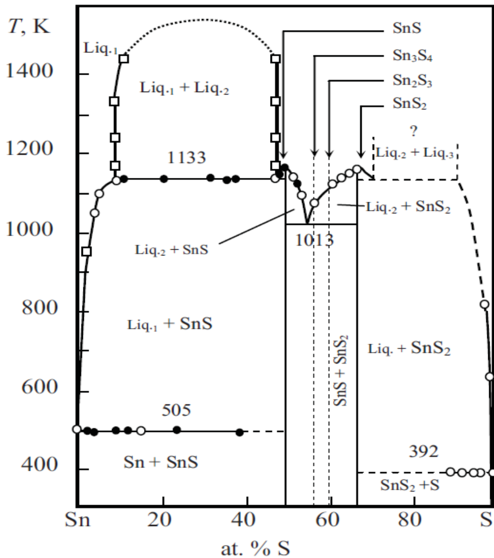
Figure S1. Sn-S binary phase diagram 1
