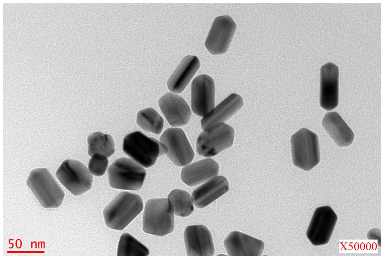
Figure S1. TEM micrograph of AgNRs after synthesis.
