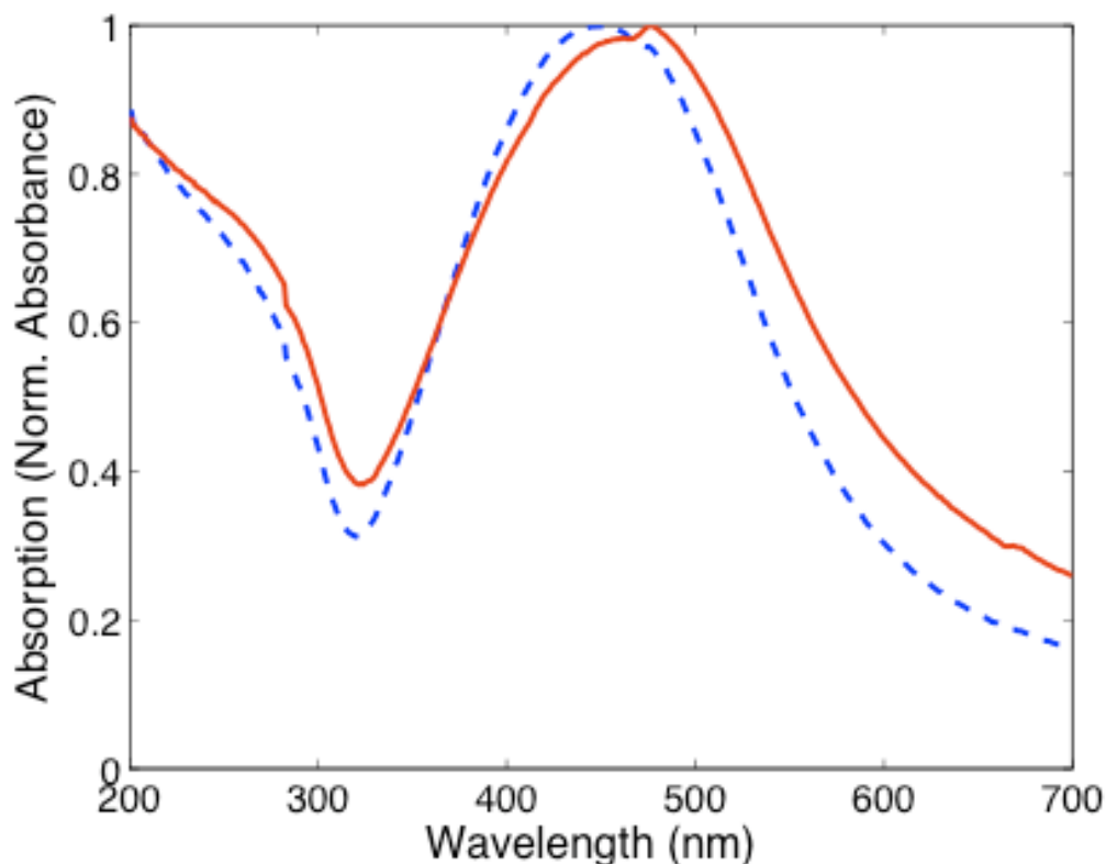
S-Figure 1 Absorption spectra of protected t -BOC Ag NP film (red solid line) before patterning and deprotected t -BOC Ag NP film (blue dashed line) after patterning.
