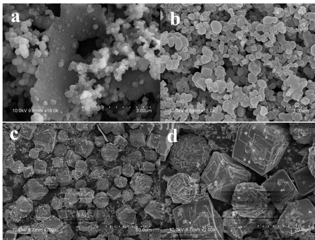
Figure S1 (a) an SEM image of the product prepared with the addition of 0.02 g of sodium gluconate but without the addition of urea; (b) an SEM image of the product prepared with the addition of 0.05 g of sodium gluconate but without the addition of urea; (c, d) SEM images of the product prepared with the addition of 0.01 g of urea but without the addition of sodium gluconate.
