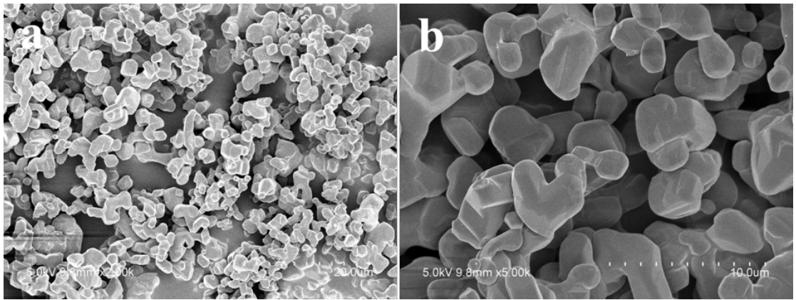
Figure S2 SEM images of the commercial Mn 3 O 4 powders.
