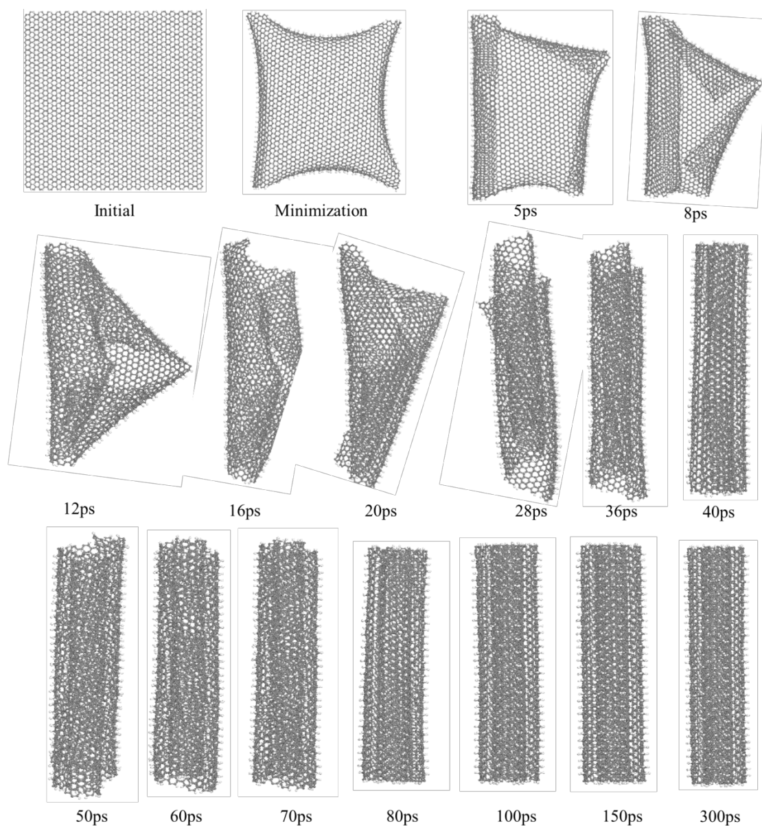
Fig. F1 shows the trajectories process of the self-assembly of C_4H from the initial sheet and after minimization to a stable state.
